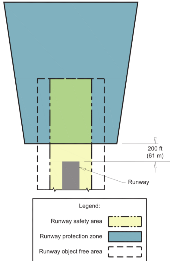
Figure 1.13 - RSA/ROFA/RPZ
