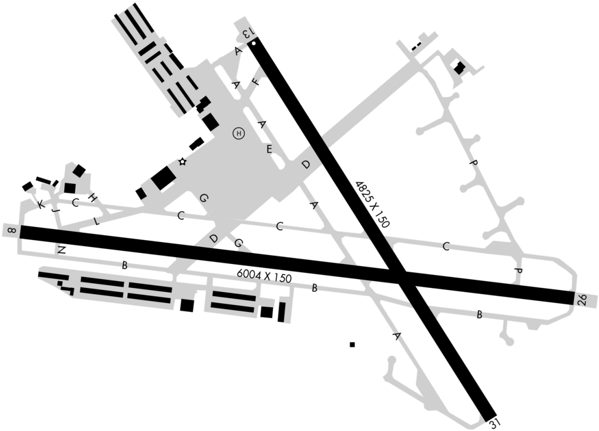
Figure 1.10 - SNS Airfield
